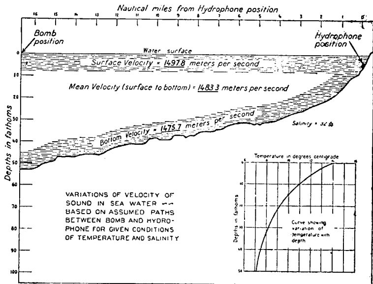
FIGURE 1. Variation of horizontal velocity of sound with assumed paths.
