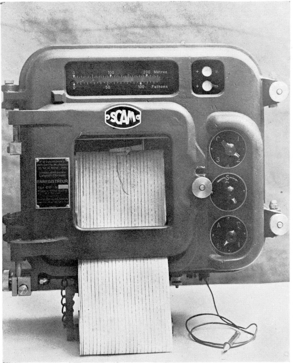
SCAM 419 Echo Sounder.
