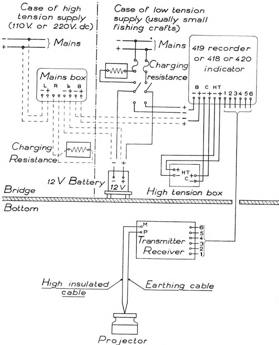
Generic Diagram of the SCAM Sounder.
