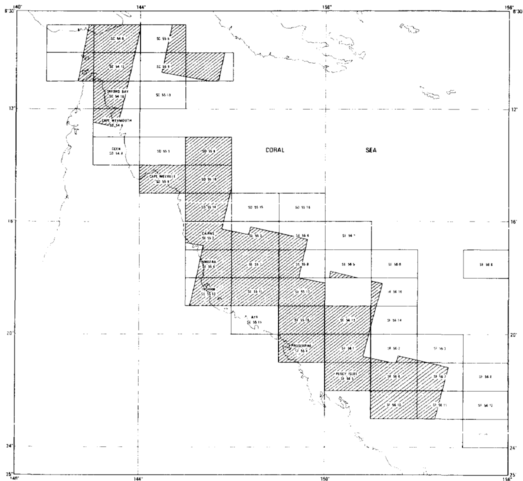
Fig. 6. — Coverage of the Great Barrier Reef by the Reconnaissance Series at 1 : 250 000 scale ; hachured areas were revised using Landsat-1 imagery.
