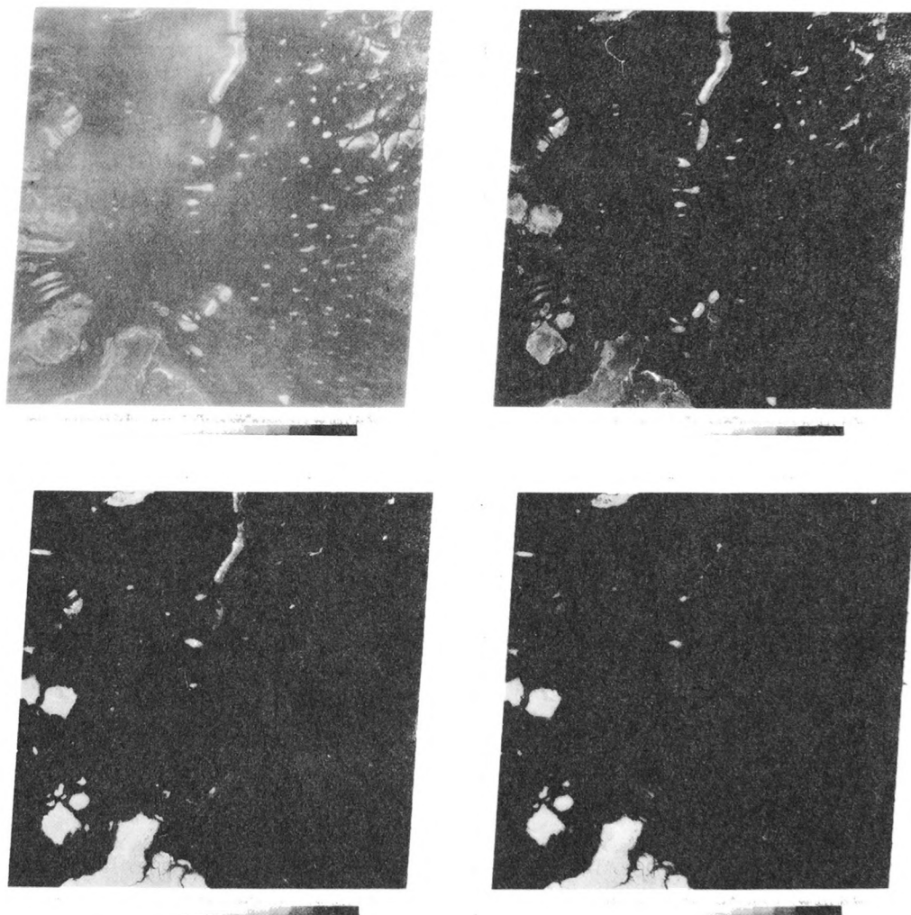
FIG. 7. — Landsat-1 scene 1026-00035 (Torres Strait) in four MSS spectral bands. Band 4, with most penetration, is shown in the top left hand frame; band 2, which has negligible water penetration, is on the lower right.
