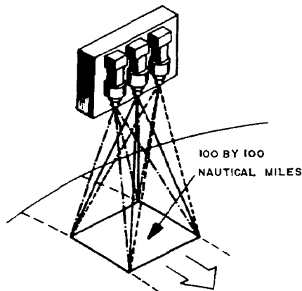
FIG. 3. — Principles of Landsat Return Beam Vidicon (after PERRY, 1972).
