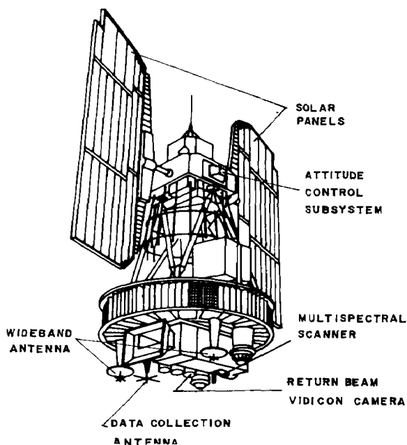
FIG. 1. — ERTS-1 (LANDSAT-1) satellite (after PERRY, 1972).
