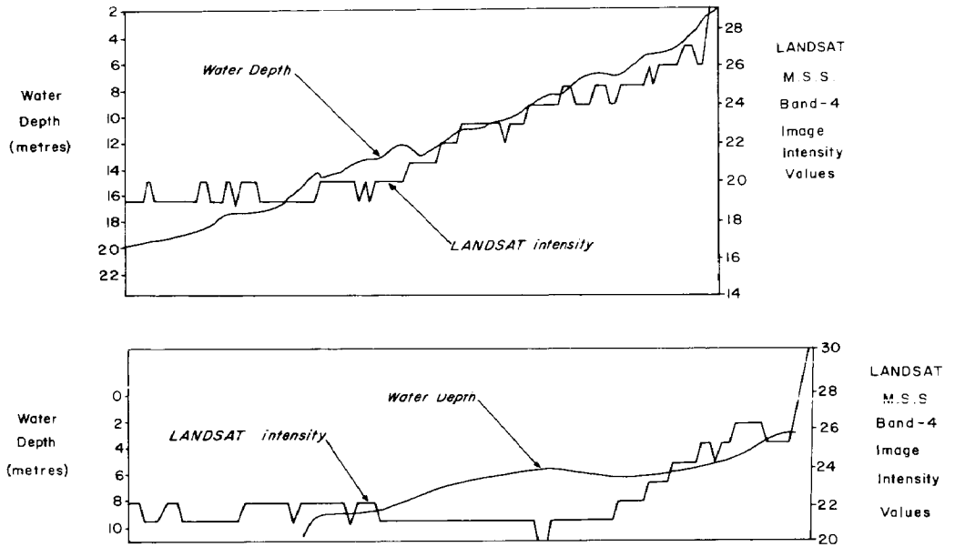
FIG. 8. — Examples of successful and unsuccessful correlation between water depths and image intensity values.
