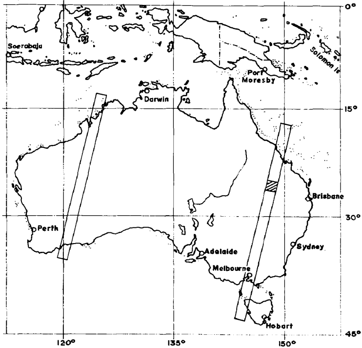
FIG. 2. — Examples of successive Landsat orbits over Australia (after PERRY, 1972).
