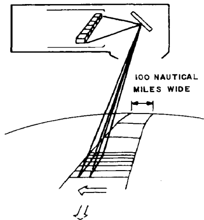
FIG. 4. — Principles of Landsat multispectral scanner (after PERRY, 1972).
