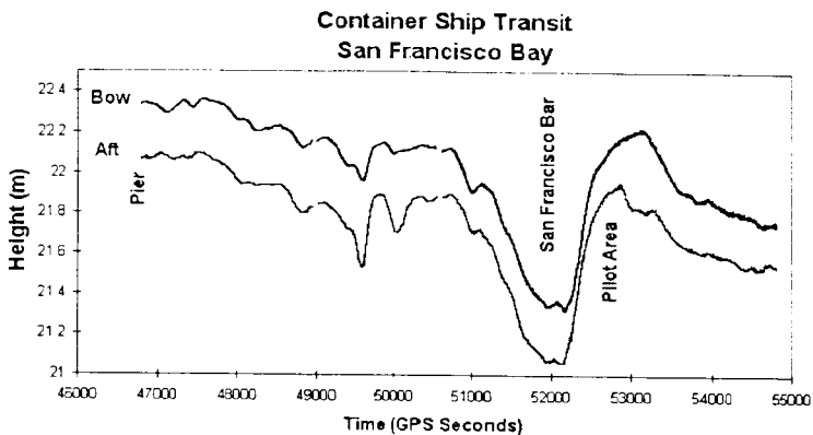
FIG 6 - Vertical trajectories for the bow and aft sections of a container ship leaving a pier in the Port of Oakland and transiting San Francisco Bay, as determined by OTF-GPS. The ship's transit covered approximately 40 km in about 2 hours.
