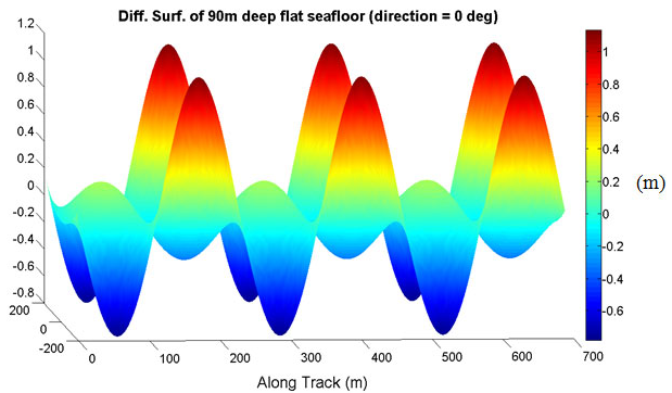
Figure 10: Difference surface of 90m deep flat seafloor (direction = 0°).
