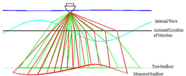
Figure 6 : True ray paths vs. traditional ray trace.
