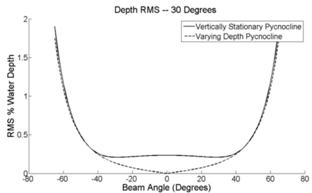
Figure 16: Depth RMS improvement by tracking velocline depth (30°).
