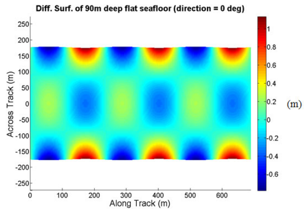
Figure 9: Difference surface of 90m deep flat seafloor (direction = 0°).
