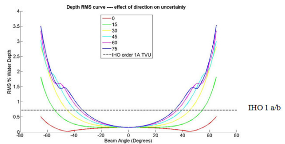
Figure 13: Depth RMS for different directions at standard
