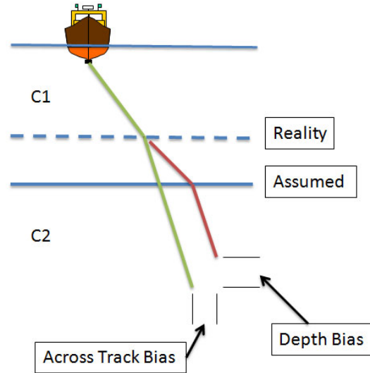
Figure 3: Effect of the velocline's vertical oscillation on MBES soundings
