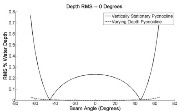
Figure 15: Depth RMS improvement by tracking velocline depth (0°).
