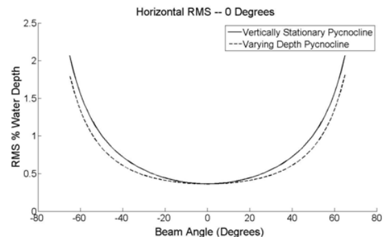
Figure 17: Horizontal position RMS improvements by tracking velocline depth.
