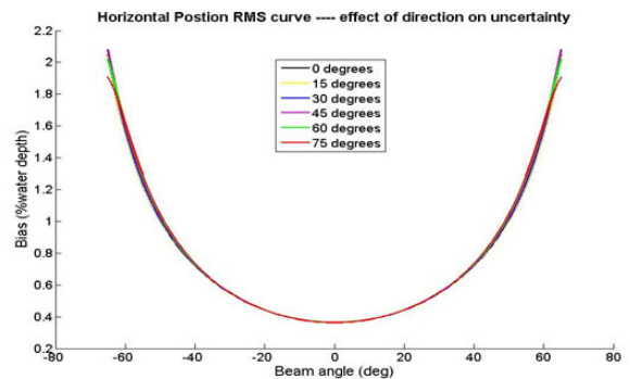
Figure 14: Horizontal positions RMS for different directions.
