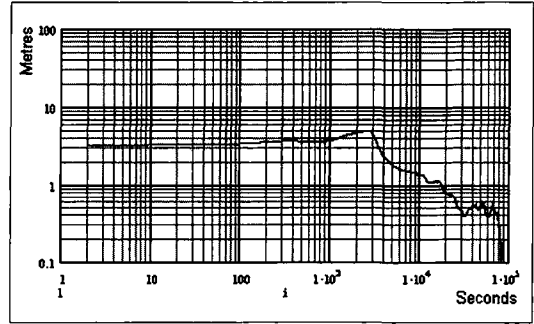
Figure 4: GPS without S.A - the effect of position averaging, logarithmic scales
