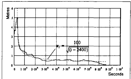
Figure 6: GPS without S.A - the effect of position averaging, linear scales
