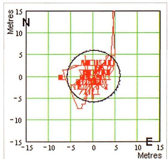
Figure 2: GPS without S.A.; CEP and error ellipse for p=0.95
