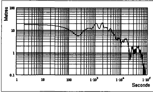
Figure 3: GPS with S.A - the effect of position averaging, logarithmic scales
