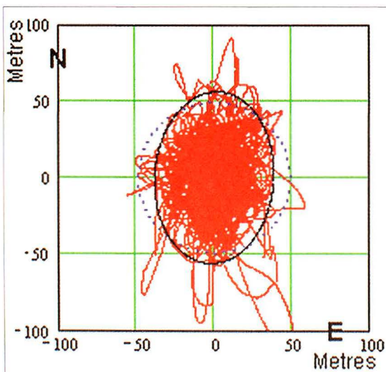
Figure 1: GPS with S.A.; CEP and error ellipse for p=0.95
