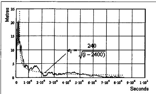
Figure 5: GPS with S.A - the effect of position averaging, linear scales
