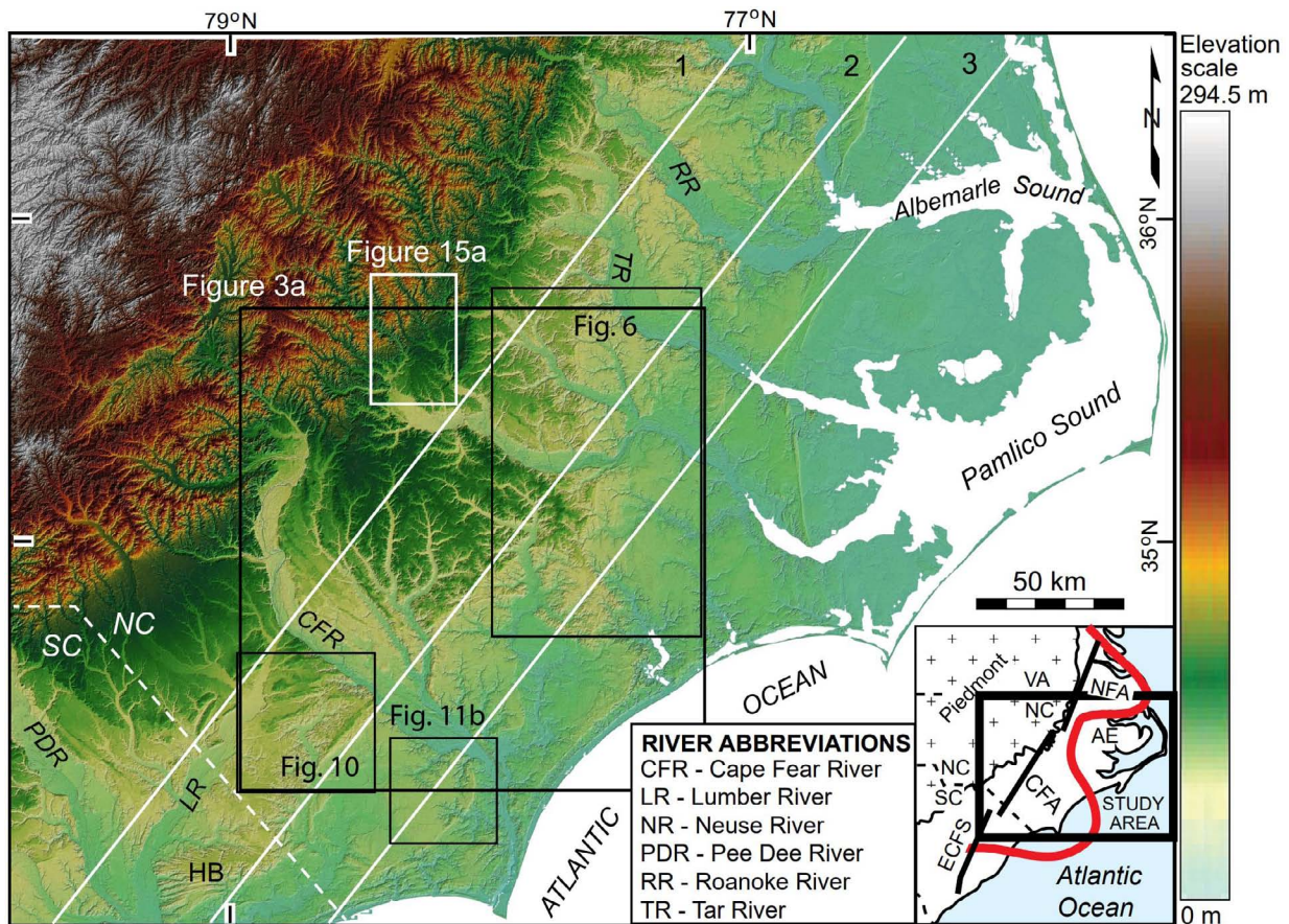
Figure 1. Regional LiDAR image across the Cape Fear arch (CFA) in the Coastal Plain of North and South Carolina. Illumination azimuth is 60^\circ . Lines labeled 1–3 are locations of elevation profiles shown in Figure 2. HB is the Horry barrier. NC – North Carolina, SC – South Carolina, VA – Virginia. Abbreviations in the index map: AE – Albemarle embayment, CFA – Cape Fear arch, ECFS – East Coast fault system of Marple and Talwani (2000), NFA – Norfolk arch.
