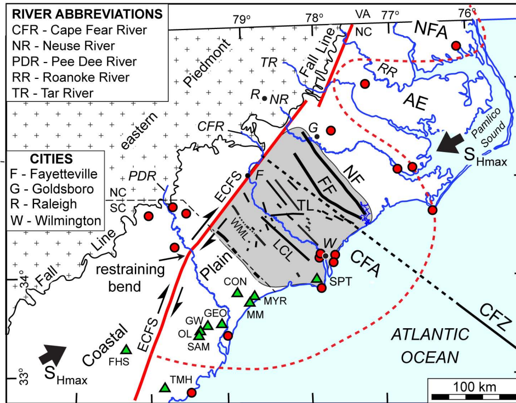
Figure 18. Conceptual diagram showing the possible relationship between the \sim 15^\circ restraining bend along the ECFS (red lines) and the area of proposed faults (black lines) along the Cape Fear arch (grey pattern). FF and NF are the interpreted Faison and Neuse faults. LCL, WML, and TL are the Livingston Creek, White Marsh, and Tomahawk lineaments. CFZ is the Carolina fracture zone (Klitgord et al. 1988) and the dashed line is the northwest projection of the CFZ. Red dots are earthquake epicenters of at least magnitude 3 (Stover and Coffman 1993). Green triangles are paleoliquefaction sites in South Carolina (CON – Conway, FHS – Four Hole Swamp, GEO – Georgetown, GW – Gapway, MM – Martin Marietta, MYR – Myrtle Beach, OL – Olin, SAM – Sampit, TMH – Ten Mile Hill) and in North Carolina (SPT – Southport) (Talwani and Schaeffer 2001). Opposing arrows labeled S_{Hmax} indicate the orientation of the maximum horizontal compressive stress field (Zoback and Zoback 1991). The dashed red contour shows the locations of the Cape Fear arch (CFA), Albemarle embayment (AE), and Norfolk arch (NFA).
