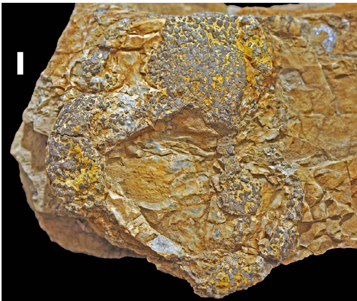
Figure 2. NBMG 16862, Scyphocrinites sp., a collapsed lobolith from the Indian Point Formation, northern New Brunswick (after Donovan and Miller 2014, fig. 4); Upper Silurian (Pridoli) or, less likely, Lower Devonian (Lochkovian). Specimen uncoated. Scale bar represents 10 mm.
