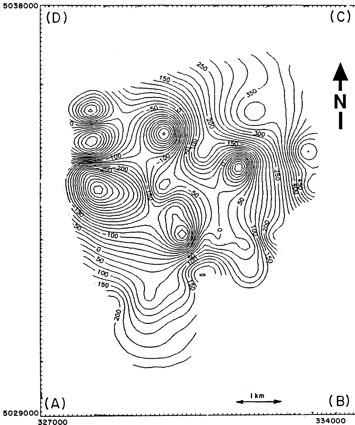
Fig. 6. Granite depth estimates (base of intrusion) within surface boundary limits and with respect to mean sea level (m.s.l.); the positive values (in m) are located above m.s.l. and the negative values below m.s.l. Contour interval is 50 m.
