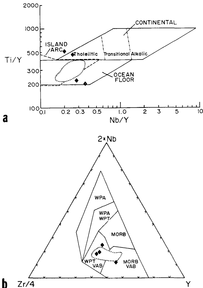
Fig. 6. (a) Plot of Ti/Y against Nb/Y for basaltic (dotted field) and gabbroic (diamonds) samples. Fields from Pearce (1982). (b) Basaltic (dotted field) and gabbroic (diamonds) samples plotted on the ternary Nb-Zr-Y diagram of Meschede (1986). Fields WPA = within-plate alkalic basalt; WPT = within-plate tholeiitic basalt; MORB = mid-ocean ridge basalt; VAB = volcanic arc basalt.
