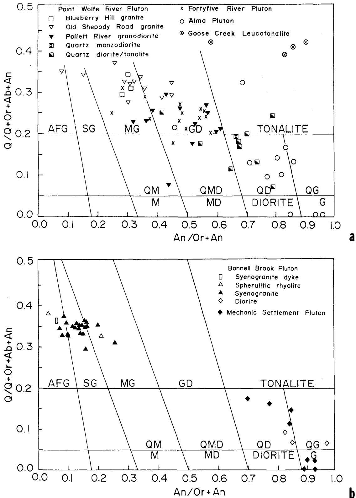
Fig. 8. Plots of CIPW normative Quartz/Quartz+Orthoclase+Albite+Anorthite against Anorthite/Orthoclase+Anorthite for plutonic rocks of the study area. Data are from Tables 3, 4, and 6, Barr (1987), and Barr and White (1988a). Fields are from Streckeisen and Le Maitre (1979); AFG = alkali feldspar granite, SG = syenogranite, MG = monzogranite, GD = granodiorite, QM = quartz monzonite, M = monzonite, QMD = quartz monzodiorite, MD = monzodiorite, QD = quartz diorite, QG = quartz gabbro, G = gabbro. (a) Older group of plutons: Goose Creek leucotonalite (n = 4), Alma Pluton (n = 11), Fortyfive River Pluton (n = 14), and Point Wolfe River Pluton: quartz diorite/tonalite (n = 9), quartz monzodiorite (n = 1), Pollett River granodiorite (n = 12), Old Shepody Road granite (n = 13), Blueberry Hill granite (n = 3). (b) younger group of plutons: Mechanic Settlement Pluton (n = 8), Bonnell Brook Pluton: syenogranite (n = 22), diorite (n = 3) spherulitic rhyolite dome (n = 2).
