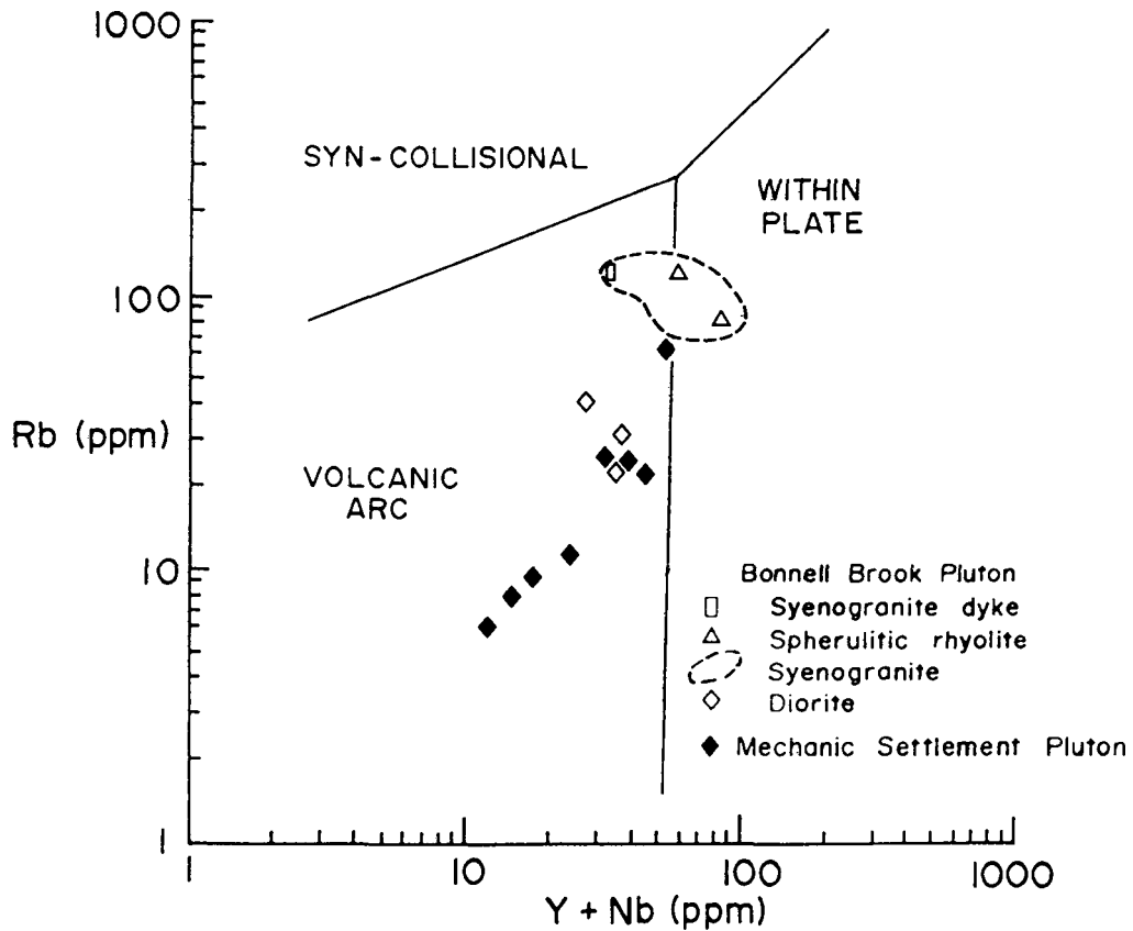
Fig. 10. Plots of Rb against Y+NB. (a) older plutons and (b) younger plutons, as in Figure 8. Fields are from Pearce et al. (1984).
