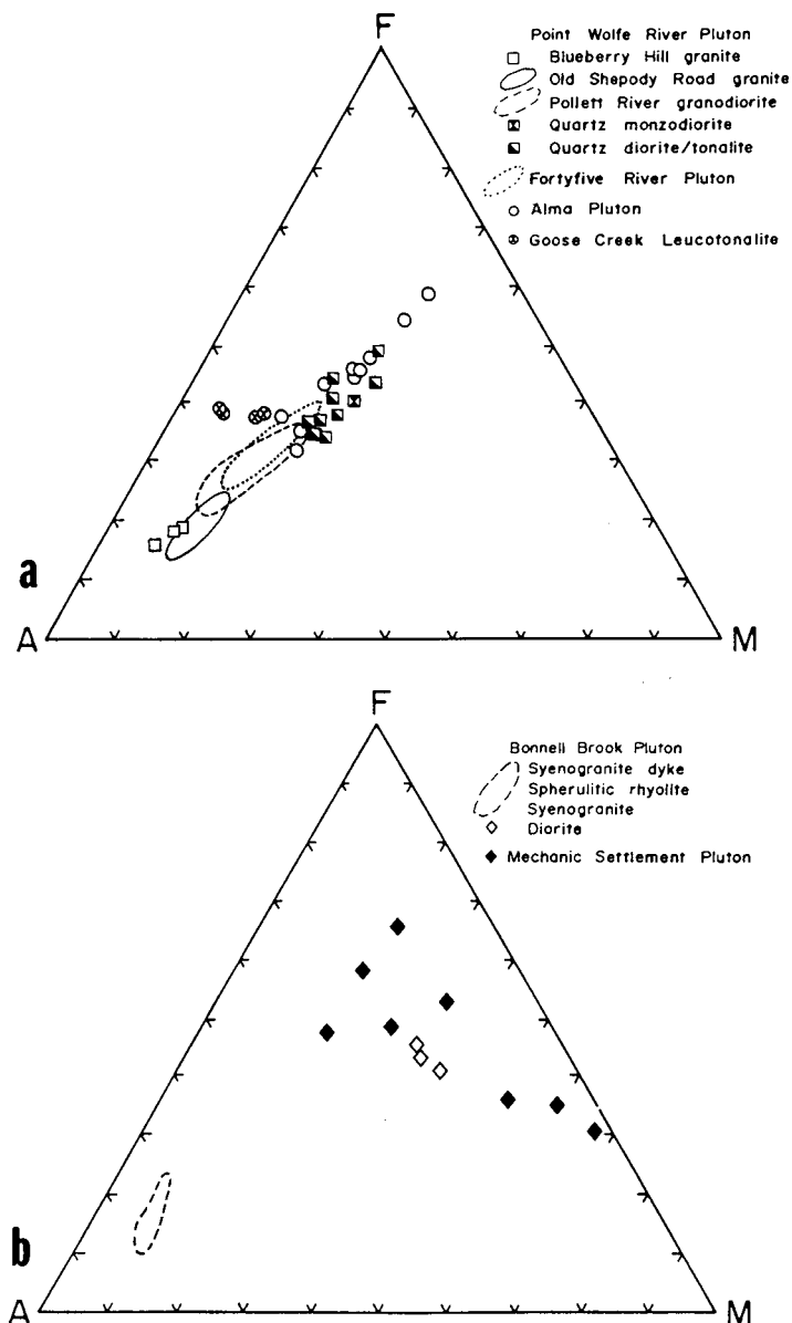
Fig. 9. A( \text{Na}_2\text{O}+\text{K}_2\text{O} ) - F(FeO total) - M(MgO) diagrams for plutonic rocks of the study area. (a) older plutons and (b) younger plutons, as in Figure 8.
