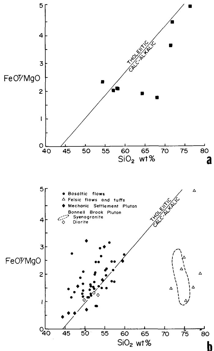
Fig. 3. Plots of FeOT/MgO against silica for (a) metatuffaceous samples from volcanic-sedimentary sequence A and (b) basaltic flows and felsic flows and tuffs from volcanic-sedimentary sequence B and samples from Bonnell Brook and Mechanic Settlement plutons. Data from Tables 1, 4 and 6, Barr and White (1988a), and Barr (1987), recalculated to 100%, volatile-free. FeOT = total iron expressed as FeO. Tholeiitic/calc-alkalic dividing line from Miyashiro (1974).
