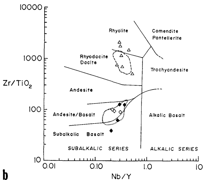
Fig. 4. Plots of Zr/TiO_2 against Nb/Y for (a) metatuffaceous samples from sequence A and (b) volcanic rocks from sequence B and Bonnell Brook and Mechanic Settlement plutons. Symbols as in Figure 3 except dotted field encloses 42 basaltic to andesitic samples from sequence B. Named fields are from Winchester and Floyd (1977).
