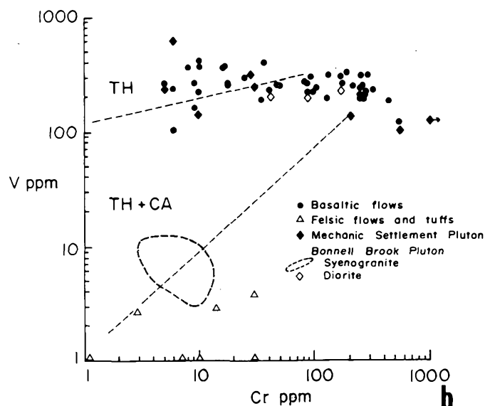
Fig. 5. Plots of V against Cr for (a) metatuffaceous samples from sequence A and (b) volcanic samples from sequence B and gabbros from Mechanic Settlement Pluton and diorite and syenogranite from Bonnell Brook Pluton. Tholeiitic (Th) and calc-alkalic (CA) fields from Miyashiro and Shido (1975).
