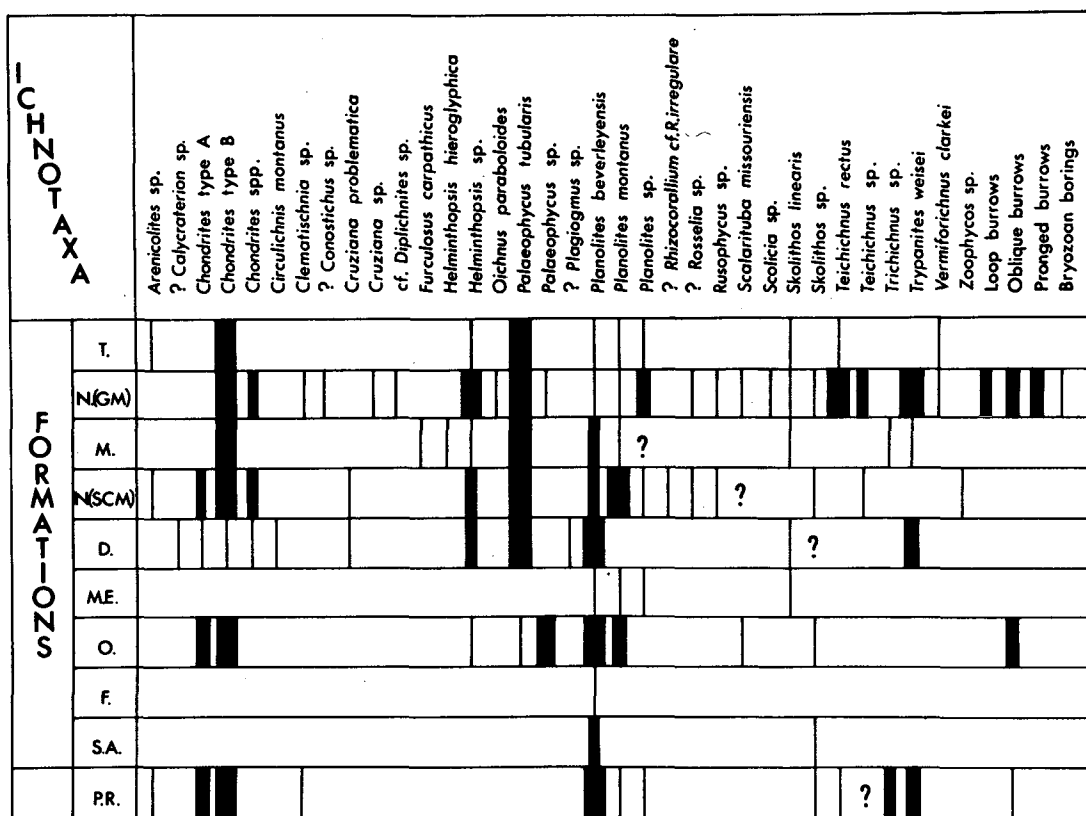
Fig. 5 - Stratigraphic distribution and abundance of trace fossils in the Trenton Group between Montreal and Quebec City. The relative bar widths represent respectively from thinnest to thickest 1<10 specimens, 10<50 specimens, 50<100 specimens and >100 specimens. Questionable occurrences refer to uncertain identifications. Formational nomenclature is P.R. = Pont Rouge, S.A. = Saint Alban, F = Fontaine, O = Ouareau, M.E. = Mile End, D = Deschambault, N(SCM) = Saint Casimir Member (Neuville), M = Montreal, N(GM) = Grondines Member (Neuville), and T = Tetreauville Formations.
