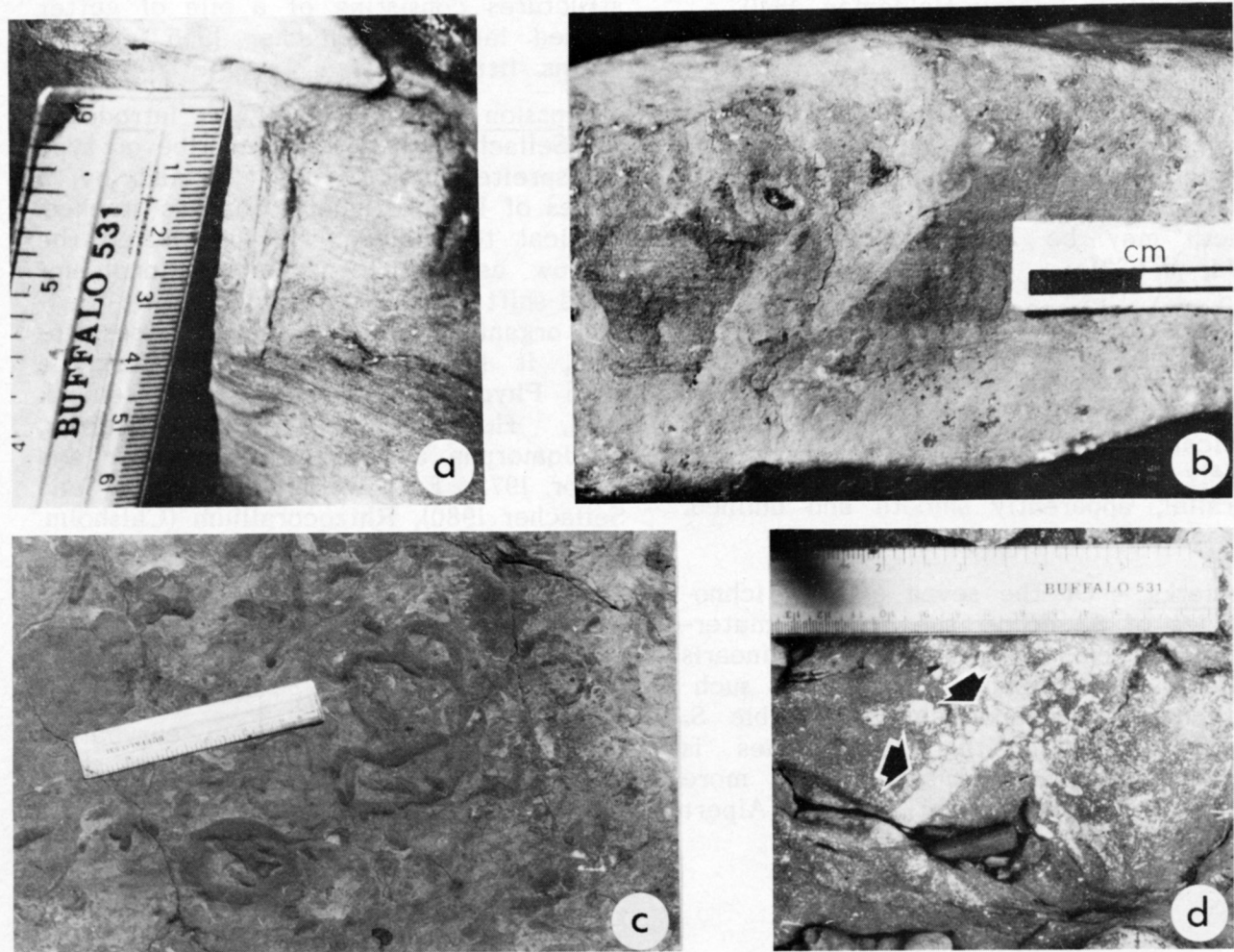
Fig. 13 - a. Skolithus linearis in vertical section, Grondines Member, locality 18. b. 'Oblique burrow' in transverse section, Grondines Member, locality 18. c. 'Loop burrows' on lower bedding surface in convex hyporelief, Grondines Member, locality 21. d. 'Pronged burrows' with typical prongs arrowed, on upper bedding surface, Grondines Member, locality 21.
