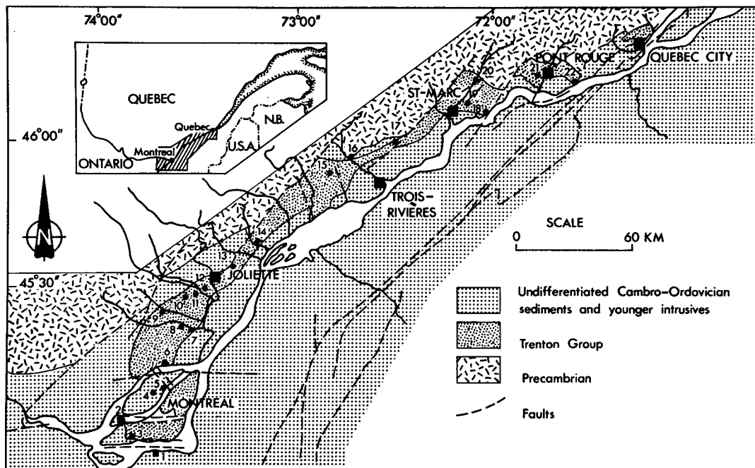
Fig. 1 - Simplified geological map of the St. Lawrence Lowland between Montreal and Quebec City. Numbered localities are: 1. Saint Constant, 2. Ile Bizard, 3. Montreal, 4. Cap Saint Martin, 5. Saint Vincent de Paul, 6. Terrebonne, 7. L'Epiphanie, 8. Saint Roch, 9. Saint Esprit, 10. Saint Jacques, 11. Highway 158/Rivière Ouareau, 12. Highway 158/Rivière Rouge, 13. Pont Corriveau, 14. Barrage savoie, 15. Pont Bournival, 16. Saint Louis de France, 17. Radnor des Forges, 18. Grondines, 19. Saint Casimir, 20. Pont Saint Alban, 21. Pont Rouge, 22. Neuville.
