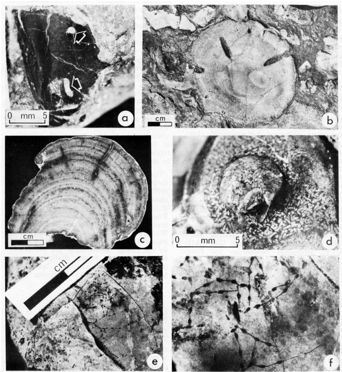
Fig. 11 - a. Oichnus paraboloides (upper arrow) and Vermiforichnus clarkei (lower arrow) in the pygidium of the isotelenid Isotelus gigas , Grondines Member, locality 18. b. Micrite filled borings of Trypanites weisei in a hemispherical colony of the bryozoan Prasopora sp., Pont Rouge Formation, locality 18. c. Longitudinal section through the bryozoan Prasopora sp. illustrating essentially vertical Trypanites weisei borings, Grondines Member, locality 18. d. Numerous small borings of Vermiforichnus clarkei in the cephalon of the isotelenid Isotelus gigas , Grondines Member, locality 18. e. f. Two views of reticulate bryozoan borings on a pygidium of the isotelenid Isotelus gigas , with f. an enlargement of the central area exhibited in e. Grondines Member, locality 18.
