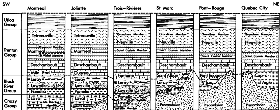
Fig. 2 - Stratigraphic profile of Middle Ordovician lithostratigraphic units between Montreal and Quebec City showing the relationship of the upper Middle Ordovician Trenton Group to underlying and overlying units. Modified after Harland and Pickerill (1982).
