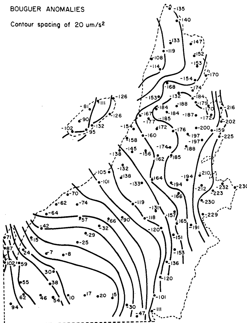
Fig. 2 - Bouguer gravity anomaly map for northeast Avalon Peninsula. Bouguer anomalies in units of \mu\text{m/s}^2 (0.1 mgals). Contour interval 20 \mu\text{m/s}^2 (2.0 mgal).
