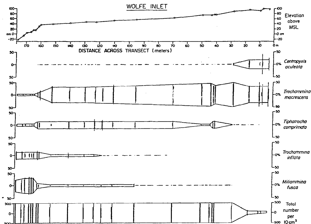
Fig. 8 - Foraminiferal distributions along Wolfe Inlet transect: Open circles are sampling localities; MSL - Benchmark MSL; double vertical bars represent the replicate samples at each locality; horizontal lines are subjective averaging (hence the vertical bars do not always fit perfectly); and, total numbers are only shown up to 1000/10 \text{ cm}^3 since all significant variations occur below this value.
