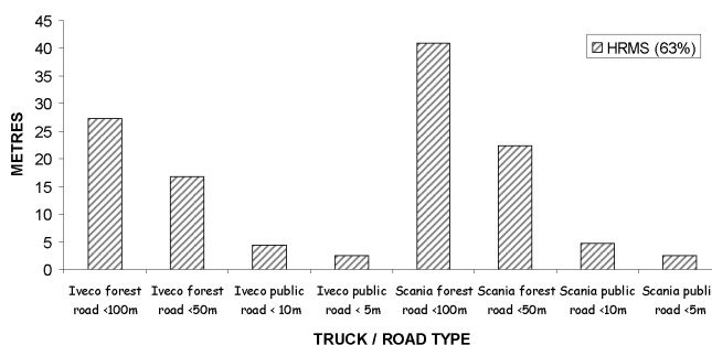
Figure 6. ~ Graph of HRMS 63% accuracy for public and forest roads for Iveco and Scania.
