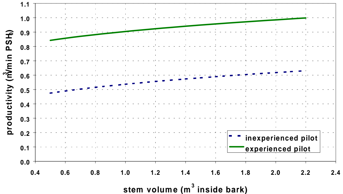
Figure 2. System productivity (m 3 /min) for the K-Max Helicopter K-Max as a function of average stem volume and pilot experience (femel cut, horizontal distance of 400 m).
