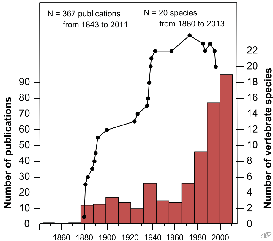
Figure 2. History of the research related to the Escuminac biota. The histogram shows the number of publications related to the Escuminac biota between 1843 and 2011. The point plot represents the discovery curve describing the number of fish species recognized in the Escuminac biota between 1880 and 2013; downward inflexion of the discovery curve corresponds to a reduction in the number of species owing to synonymization of taxa.
