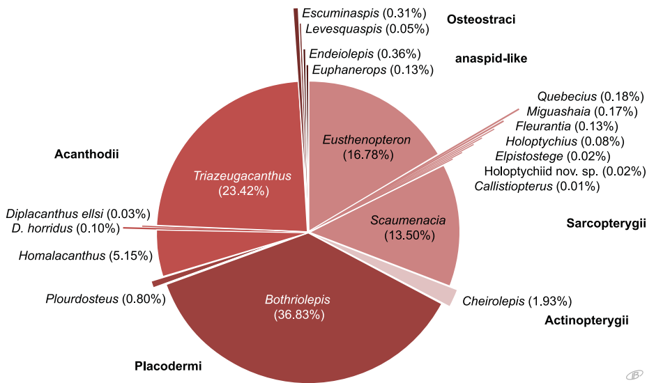
Figure 6. Relative abundance of the Escuminac fish species. The relative abundance (in %) corresponds to the proportion of the total of 18,059 specimens. Original data are provided in Cloutier et al. (2011). Bothriolepis , Triazeugacanthus , Eusthenopteron and Scaumenacia are clearly the most abundant taxa.
