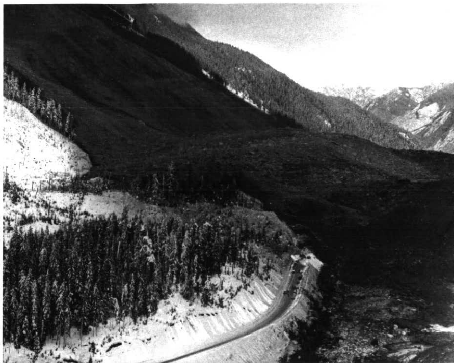
Figure 3 An example of a Geoscape image that highlights the "familiar": the 1965 Hope landslide ( Vancouver Sun )
