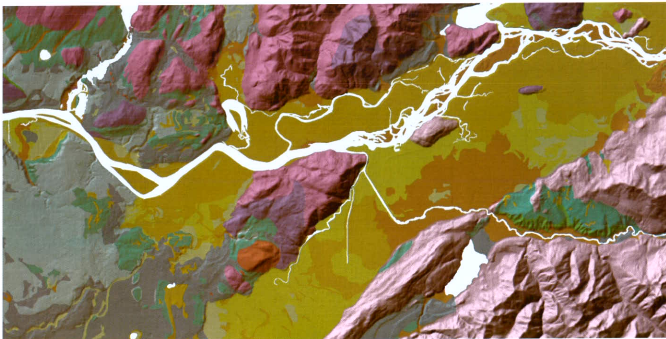
Figure 8 A portion of GeoMap Vancouver showing the value of a shaded-relief map as a base for displaying surface geology.
