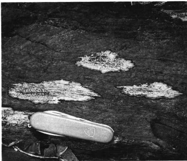
Figure 14 Fracture-oriented lichen growth along cleavage planes in a metaconglomerate near Noranda, Quebec. In this instance, the fractures have influenced thallus shape.
