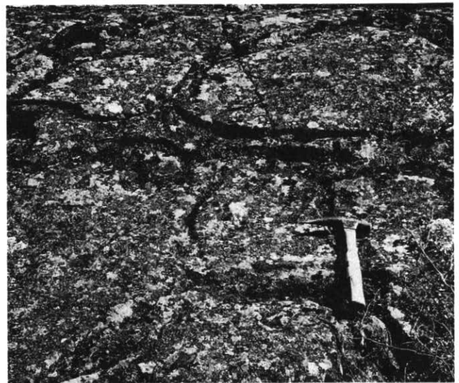
Figure 15 Umbilicaria sp. growing along pillow selvages in a pillowded, andesite flow, Back River area, Northwest Territories.
