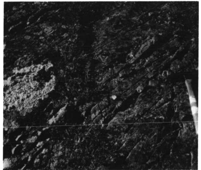
Figure 11 Contrasting lichen floras on a gabbro dyke (1 metre wide) and a feldspar porphyritic andesite. Note abundance of Lecanora argopholis (large lichen, left centre) on the andesite and its absence on the gabbro. Back River area, Northwest Territories. Table 4 summarizes the lichen species on the dike versus the andesite.
