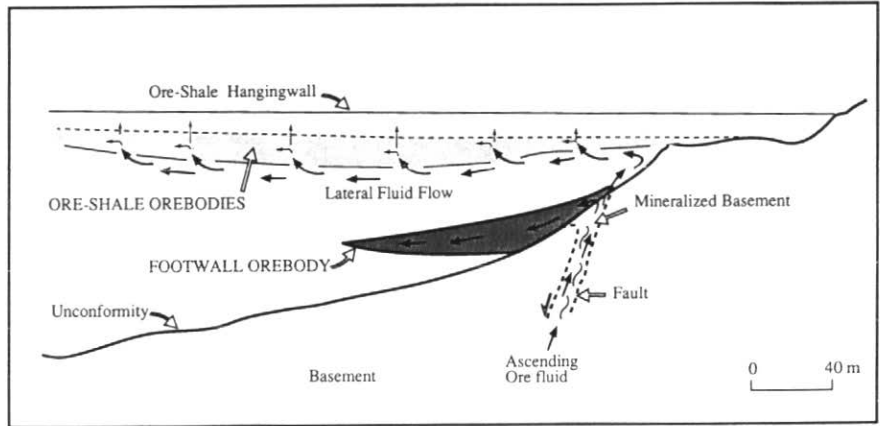
Figure 9 Interpretative diagram depicting the mineralization process for Footwall and Ore-shale orebodies in the Zambian copperbelt. Modified after Annelis (1989).
