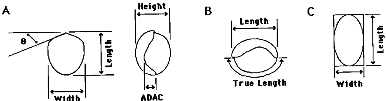
Figure 1 (A) Definition of parameters that have been used in the statistical analysis of the brachiopod Atrypa species. (After Jones, 1974). (B) Comparison of straight line measurement of shell length (L) as opposed to true length measured along shell surface (TL). (C) Diagrammatic illustration of a rectangle and an ellipse that have the same length/width ratios.
