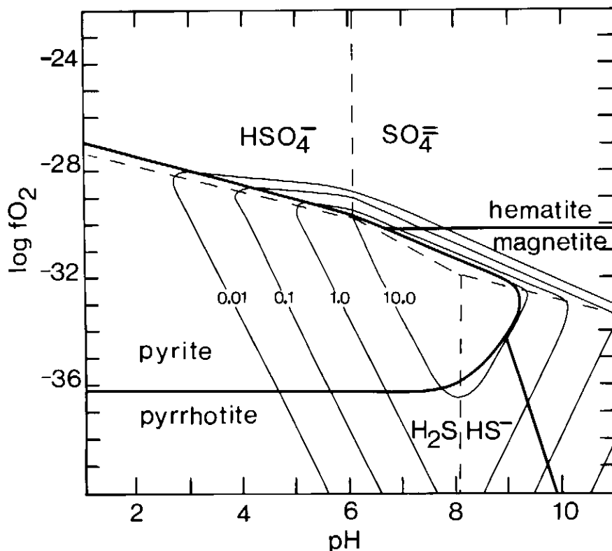
Figure 11 Calculated gold solubilities as a function of pH and log fO 2 . Gold in the thio-complex Au(HS) 2 - . Contours are in ppm. Temperature: 300°C; total sulphur 0.05 m. (Data from Seward, 1973 and 1984).
