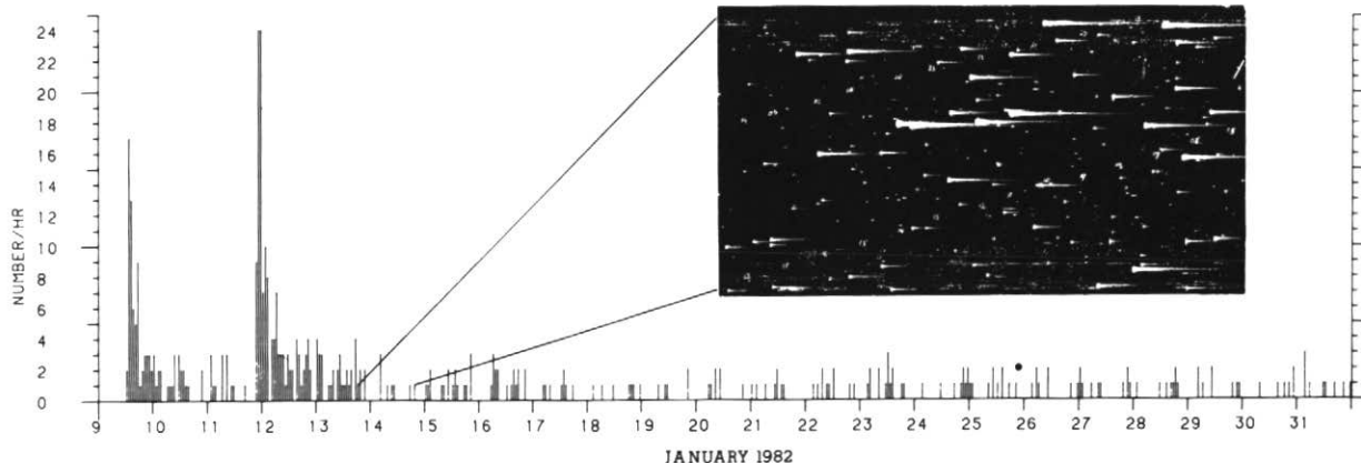
Figure 3 Number of Miramichi earthquakes per hour detected at EBN seismograph station
