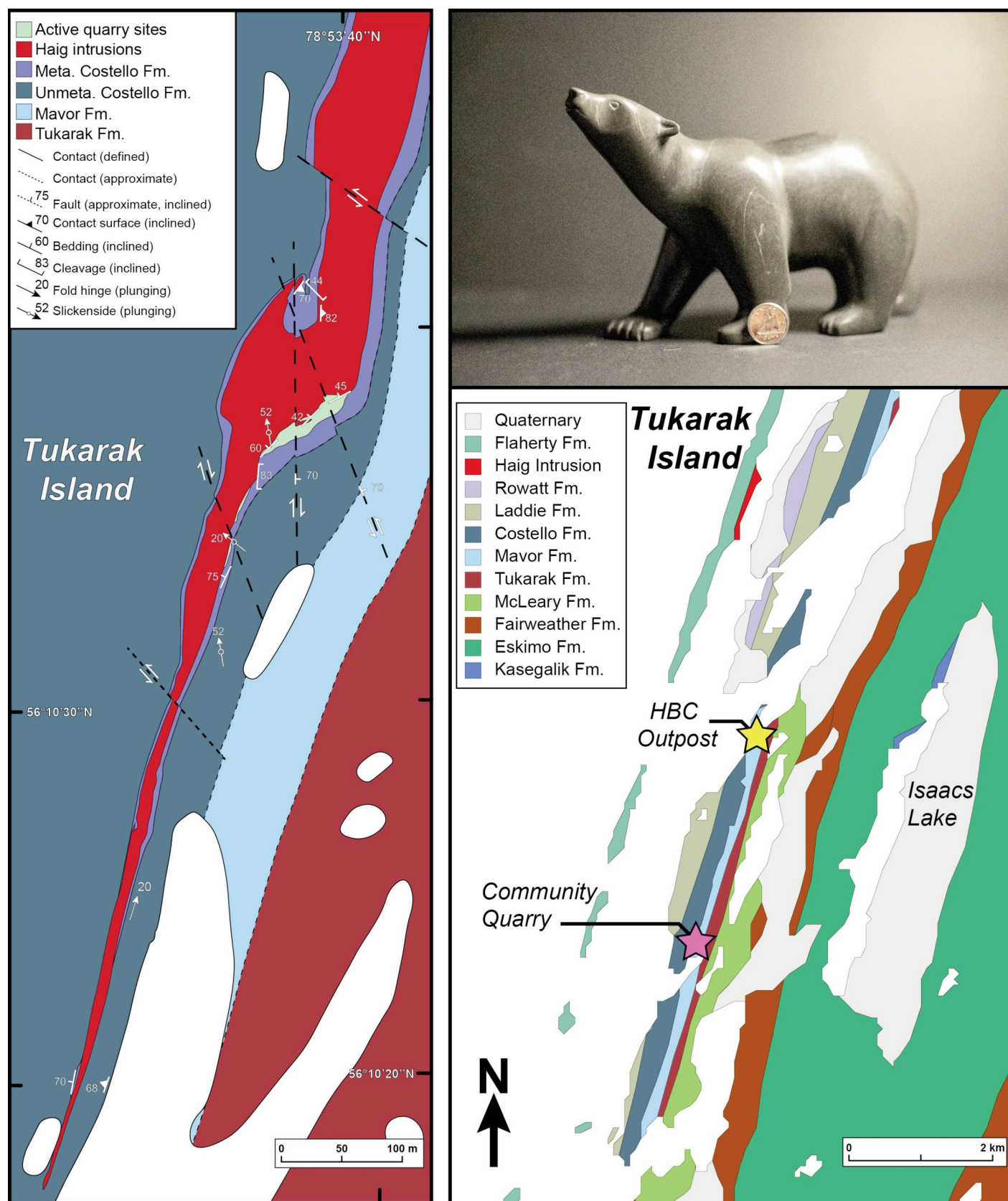
Figure 19. Detailed geological map (left) of the community quarry by Steenkamp et al. (2016); a carving of a polar bear made in 2019 by Samwillie Amagualik from carving stone developed at the contact of the Costello Formation and gabbro of the Haig Intrusion; and a geological map (right), modified from Steenkamp et al. (2016), showing the location of the old Hudson Bay Company outpost (yellow star) and the community quarry (pink star).
