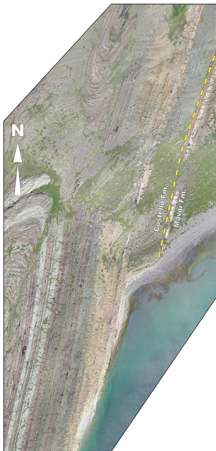
Figure 10. Drone photomosaic of the Costello Formation on southeastern Mavor Island (location indicated in Figure 2) illustrating both the poor exposure of the lower shale beds (immediately above the Mavor–Costello contact) as well as the stark colour contrast between the buff-coloured beds of the lower 100 m and the maroon-coloured beds of the upper beds.
