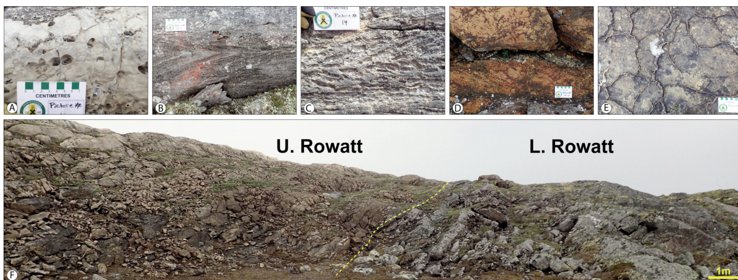
Figure 13. Compilation of main Rowatt Formation sedimentary structures and rock types. A, typical grainstone facies at the base of the upper member; B, trough cross-bedded sandstone found near the base of the formation; C, conglomerate facies preserving cross-stratification; D, clasts of dolomicrite surrounded by a silty dolomicrite matrix found within a conglomerate bed near the contact between the middle and upper zones of the lower member; E, desiccation cracks along a bedding surface; F, outcrop image facing south depicting the distinct colour difference between the upper (left) and lower (right) members.
