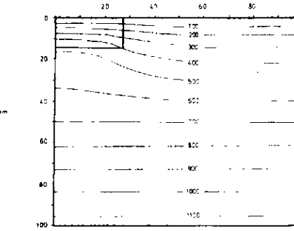
2e Granitic intrusion after 5 Ma.
