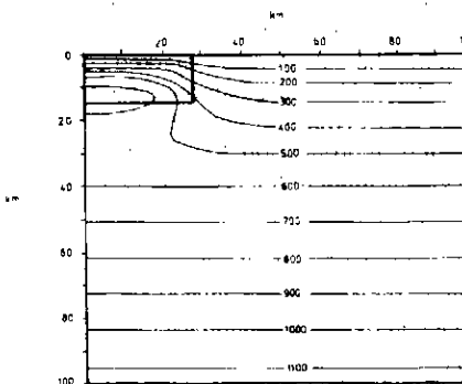
2d Granitic intrusion after 2 Ma.
