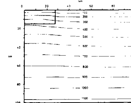
2f Granitic intrusion after 20 Ma.
