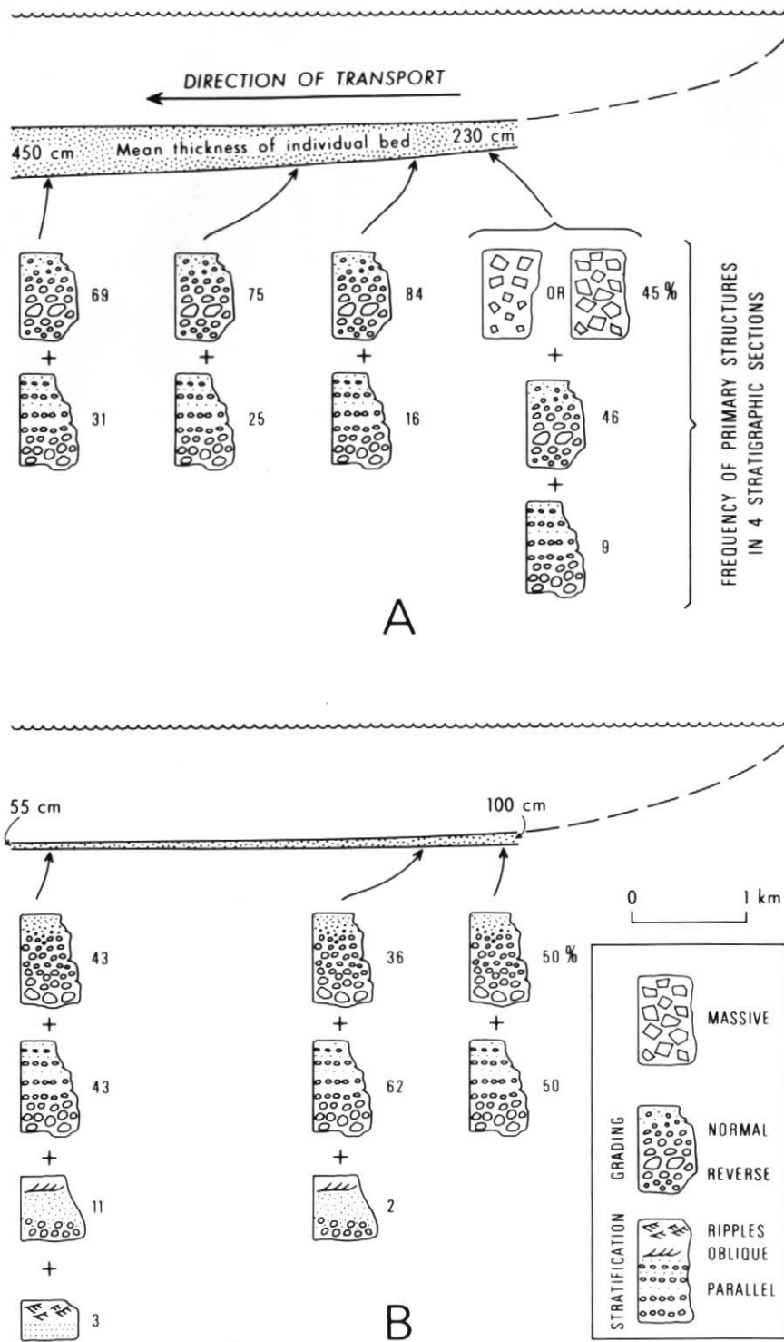
Figure 17 Lateral variations of mean bed thickness and primary structure sequences with distance of transport, in an Archean subaqueous pyroclastic flow deposit, for two different types of
