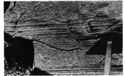
Figure 18 Primary-structure sequence in a type B bed, Rouyn-Noranda. From Tassé et al. (1978).
