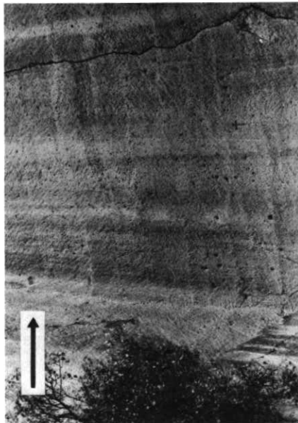
Figure 10 Stratification in air-fall deposits. A: Crude bedding, La Palma, Canary Islands. Notebook is 20 cm long. B: Crude laminations, San Lorenzo de Gran Canaria, Canary Islands. Arrow is 50 cm.
