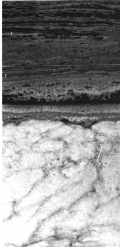
Figure 10 Upper part of sabkha cycle illustrated in Figure 9. Mosaic anhydrite cut across by erosion surface and surmounted by laminated micrites (with late-diagenetic anhydrite) of next lagoonal member. Frobisher Evaporite, Saskatchewan. Core is 11 cm across.
