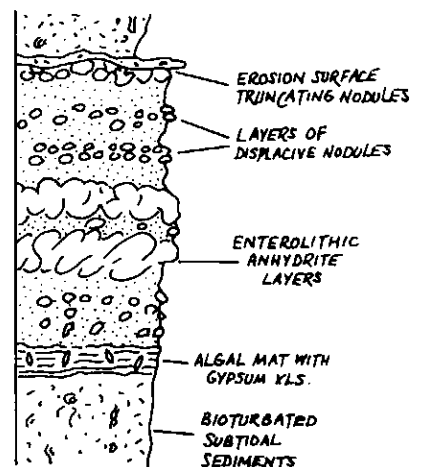
Figure 8 Characteristic features of coastal sabkha evaporites (after Shearman, 1966).
