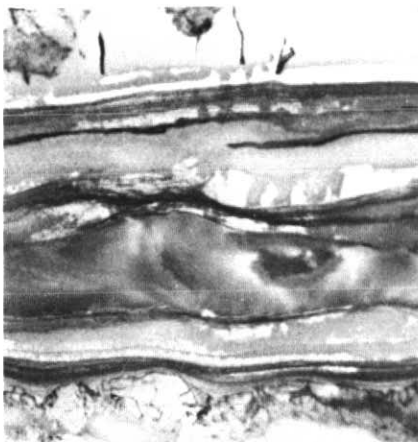
Figure 9 Laminated microlaminations (probably hypersaline lagoonal) overlain by algal mat, with gypsum pseudomorphed by anhydrite, and nodular and mosaic coastal sabkha anhydrite. Frobisher Evaporite (Mississippian) Saskatchewan. Core is 11 cm across.
