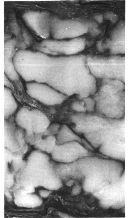
Figure 11 Mosaic anhydrite (displacing subaqueous laminated anhydrite) with individual nodules distorted against each other (a natural consequence of displacive growth). Ordovician Stonewall Evaporite, Saskatchewan. Core is 10 cm across.
