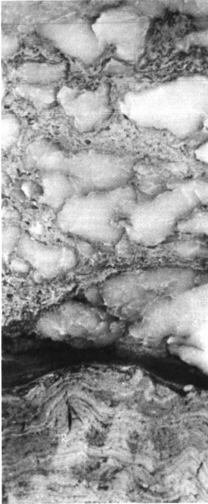
Figure 10 Upper part of sabkha cycle illustrated in Figure 9. Mosaic anhydrite cut across by erosion surface and surmounted by laminated micrites (with late-diagenetic anhydrite) of next lagoonal member. Frobisher Evaporite, Saskatchewan. Core is 11 cm across.
