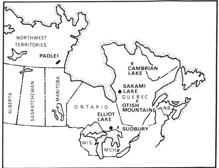
Figure 3 Basal Aphebian quartz-pebble conglomerates in Canada.
