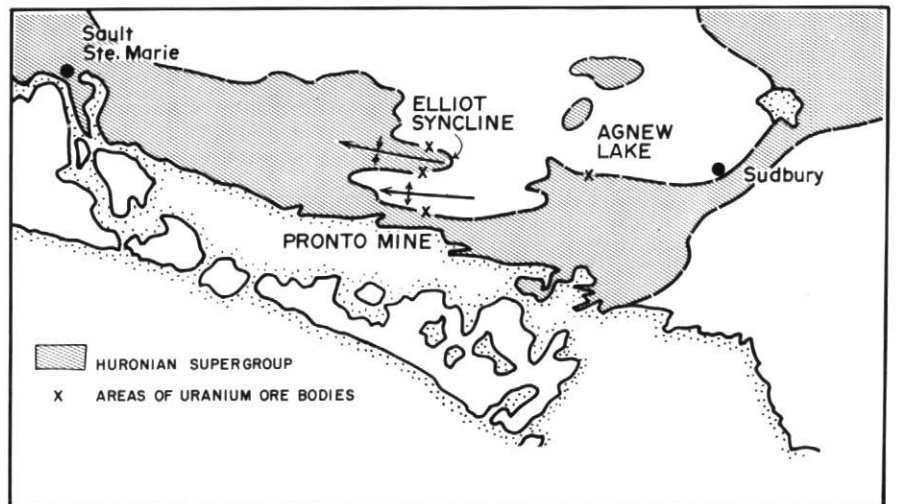
Figure 4 Huronian of the North Shore, Elliot Lake area.
