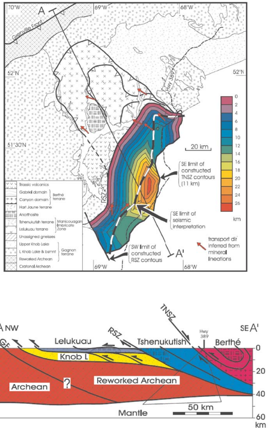
Figure 16. (a) Isopach map for the Tshenukutish terrane. Heavy dashed line is the southeastern limit of structure contours for which their position is constrained by observed reflectors. Red arrows show inferred transport directions for rocks within Tshenukutish terrane based on the predominant trends of mineral lineations. AA' is location of section below. (b) Vertical cross-section along line AA' (Figs. 15a, 16a). Depths of boundaries within the triangular field beneath the surface trace of Highway 389 are constrained by structure-contour maps derived from interpretation of Line 55. Outside that region, subsurface structure is based on extrapolation parallel to the regional tectonic trend of the Grenville orogen. Colour and ornament same as Figure 15a. From Hynes et al. (2000).
