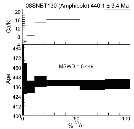
Figure 7. ^{40}\text{Ar}/^{39}\text{Ar} step-heating spectrum (all steps are presented at 2\sigma relative uncertainties) and ^{37}\text{Ar}_{\text{Ca}}/^{39}\text{Ar}_{\text{K}} ratio diagram of East Pond Metamorphic Suite amphibolite sample 08SNB-T130. Plateau age uncertainty is 2\sigma and includes both analytical and J-factor error. See Figure 1 for sample location. MSWD: mean square of weighted deviates.
