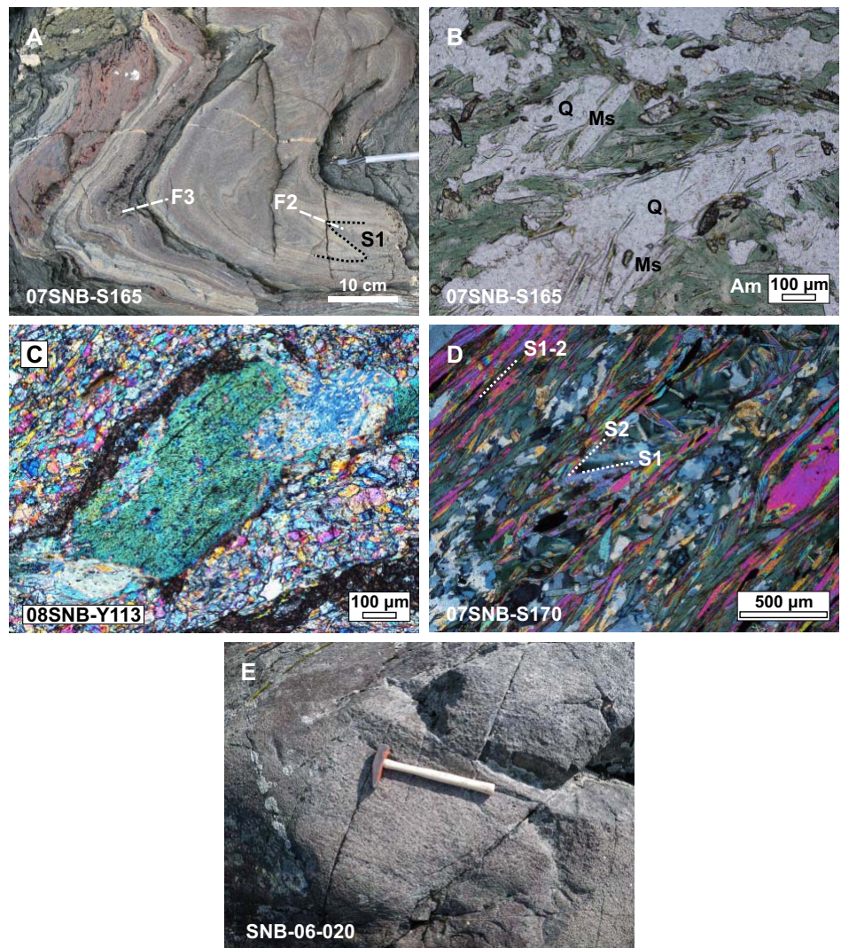
Figure 3. Representative photographs of dated Birchy Complex (A to D) and eclogite (E) localities and thin sections. A: Complexly folded (F 2 and F 3 of predominant S 1 ) mafic schist with lenses of jasper and epidosite (sample 07SNB-S165). B: Photomicrograph (plane-polarized light) of sample 07SNB-S165 showing epidote- and hornblende-bearing mafic schist, with possible quartz-muscovite veinlets. Am: Amphibole; Ms: Muscovite; Q: Quartz. C: Photomicrograph (crossed polars) of a typical amphibole porphyroblast of the gabbro sample 08SNB-Y113. D: Photomicrograph (crossed polars) showing the strongly developed S 2 fabric overprinting S 1 , only locally differentiated, from the psammite sample of locality 07SNB-S170. E: Dated eclogite body along the north end of Gull Pond (Hibbard 1983). Retrogression of the weakly foliated eclogite to amphibolite is moderate, but becomes progressively more pronounced towards the contact with the strongly foliated enveloping gneiss and schist of the East Pond Metamorphic Suite. The amphibolitized eclogite is interpreted as a polymetamorphosed mafic dyke. See Figures 1 and 2 for sample locations.
