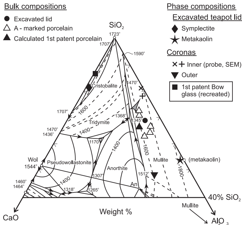
Figure 6. Displacement of melt compositions (see grey arrow) away from the 1345°C eutectic on the \text{SiO}_2\text{--CaO--Al}_2\text{O}_3 phase diagram (Osborn and Muan 1960). The melt phase, represented by inner (glass) coronas in this 1 st patent ('A-marked') Bow porcelain teapot lid, changed to more Ca-poor compositions as labradorite in the surrounding (outer) corona (Fig. 5) formed. Modified after Owen (2012).
