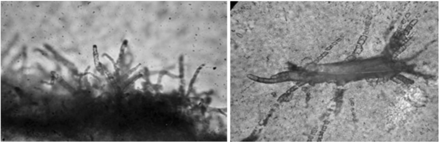
Figure 4. SEM images of tubular structures of inferred microbial origin. The image on the left is a sample from modern oceanic crust, whereas the image on the right was preserved in ancient crust. Each of these images is approximately 350 micrometers in width. Images courtesy N. Banerjee.
