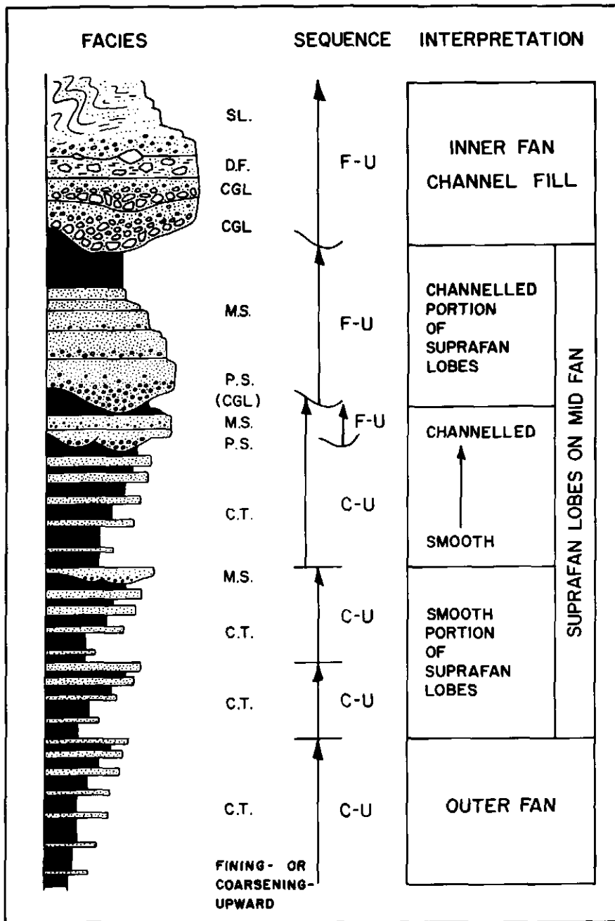
Figure 14 Hypothetical submarine fan stratigraphic sequence produced by fan progradation. C.T., classical turbidite; M.S., massive sandstone; P.S., pebbly sandstone; D.F.,
