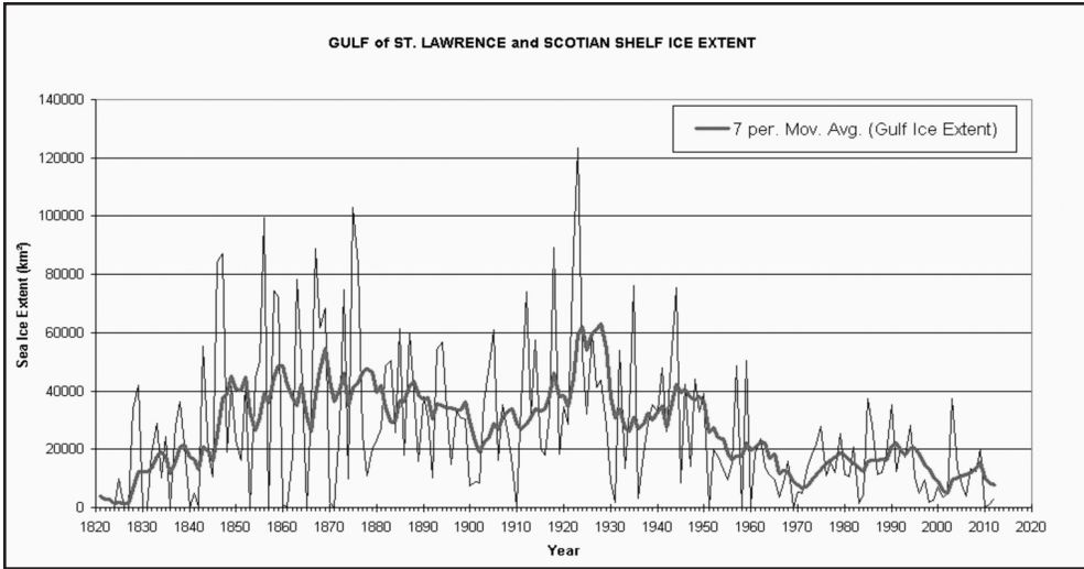
Figure 1: Gulf of St. Lawrence and Scotian Shelf Ice Extent.
