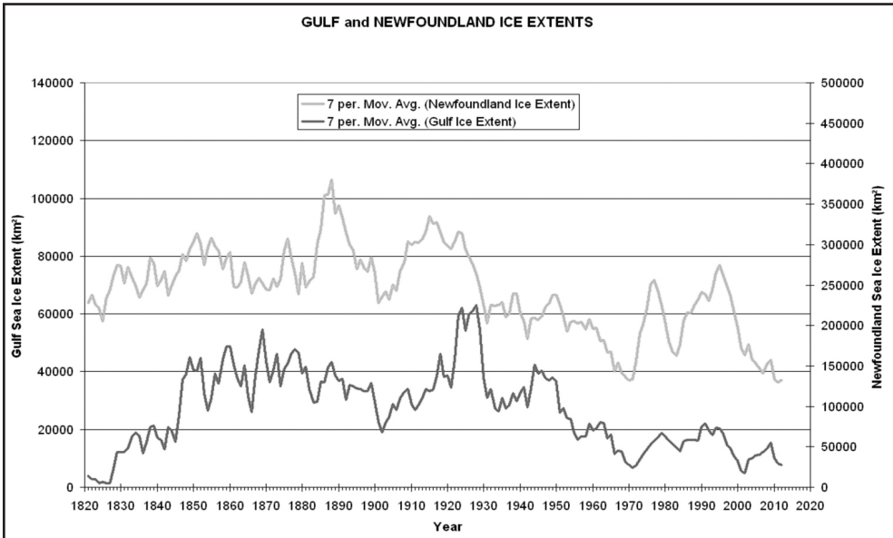
Figure 2: Gulf and Newfoundland Ice Extents.
