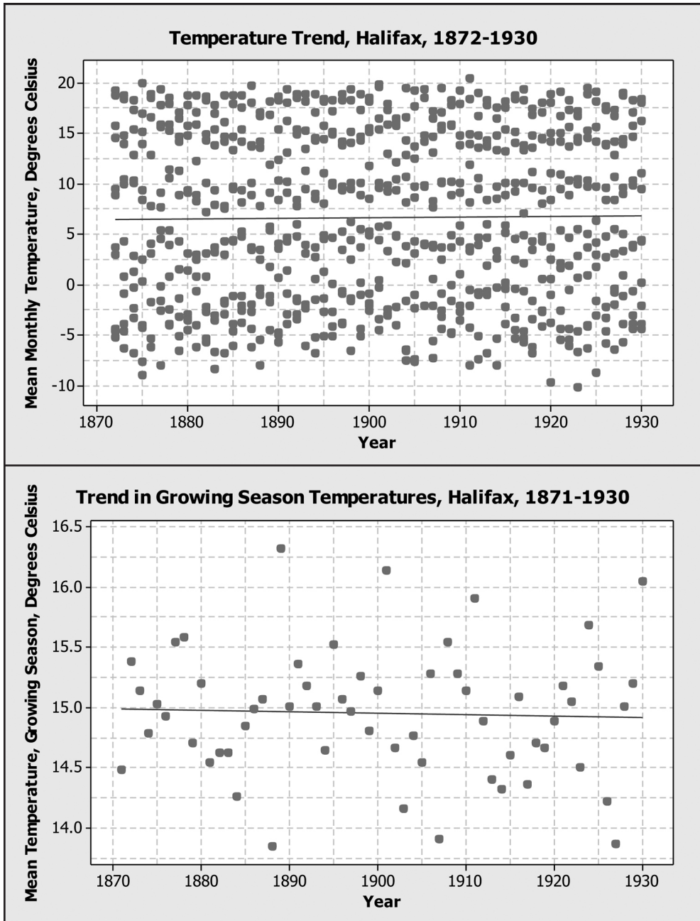
Figure 7: Temperature Trend, Halifax, 1872-1930 & Trend in Growing Season Temperatures, Halifax, 1871-1930.
